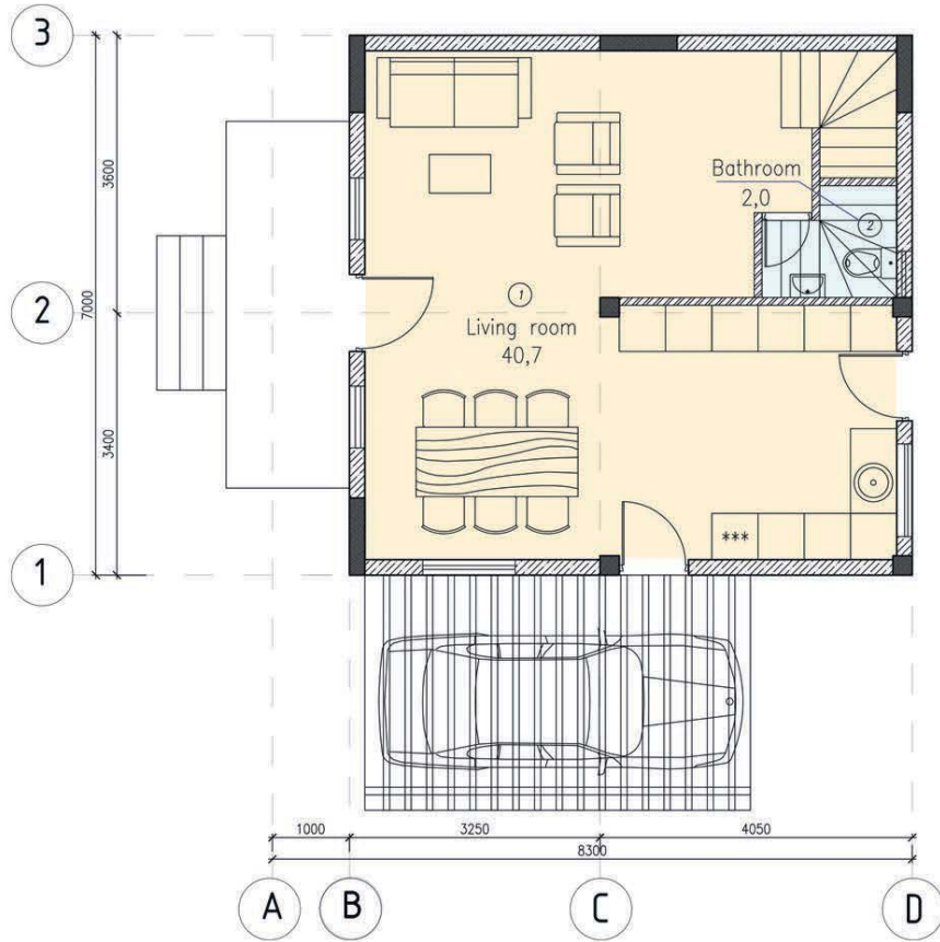
House 1. Floor plan 1
