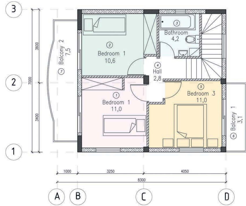
House 1. Floor plan 2
