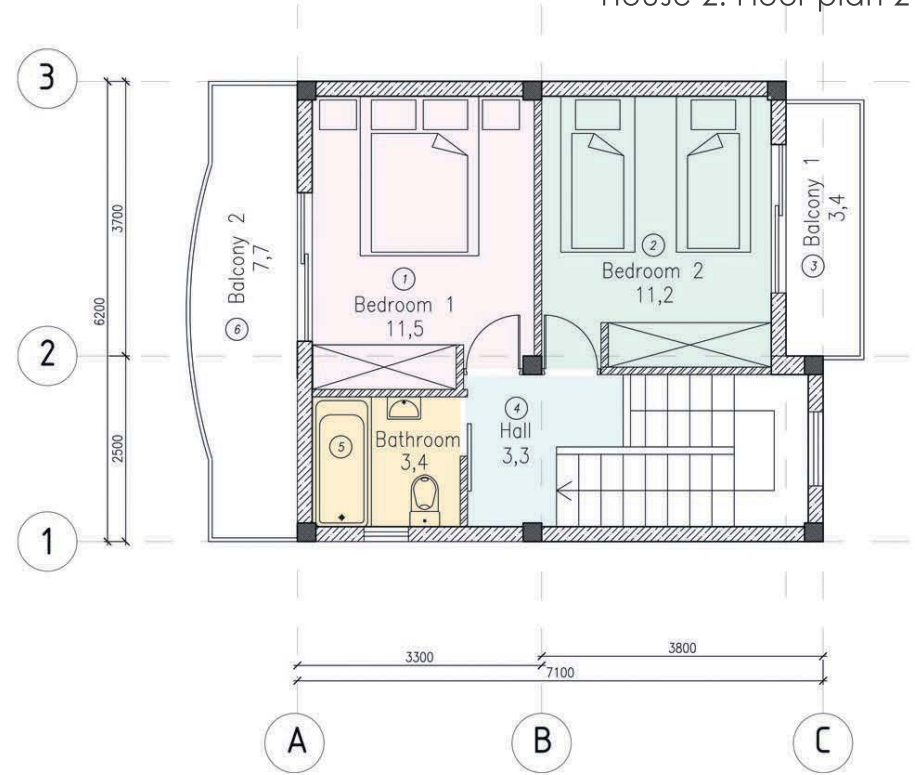
House 2. Floor plan 2
