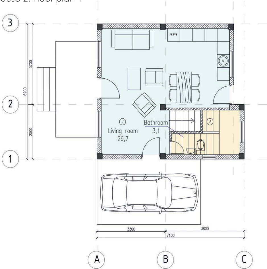
House 2. Floor plan 1
